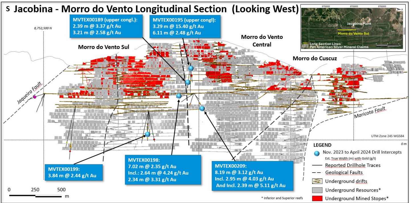
Figure 4. Jacobina – Morro do Vento Longitudinal Section (Looking West)
