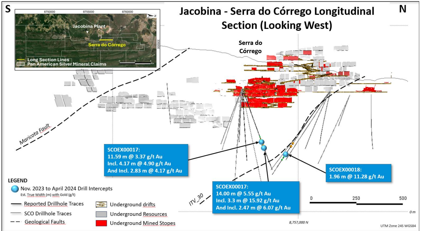
Figure 3. Jacobina – Serra do Corrego Longitudinal Section (Looking West)
