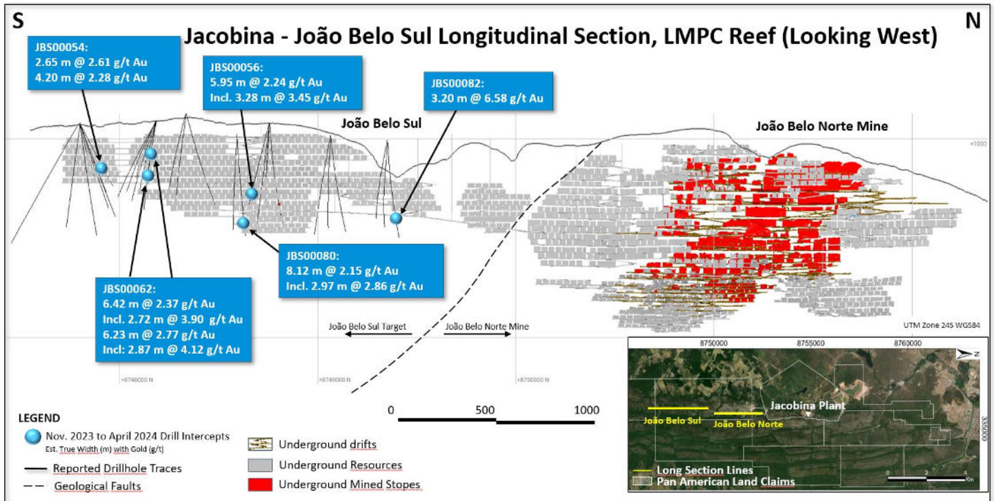
Figure 1. Jacobina – Joao Belo Sul Longitudinal Section, LMPC Reef (Looking West)
