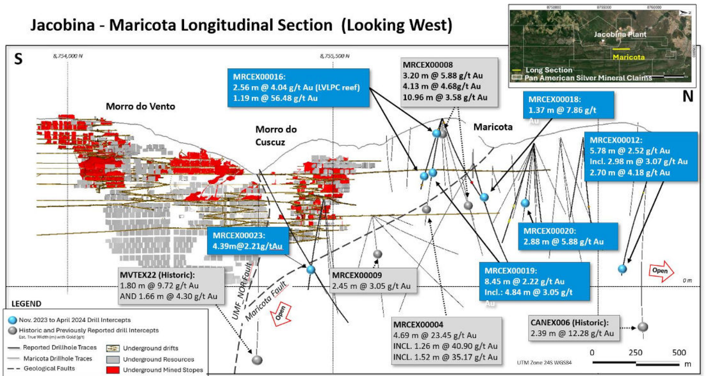
Figure 2. Jacobina – Maricota Sul Longitudinal Section (Looking West)
