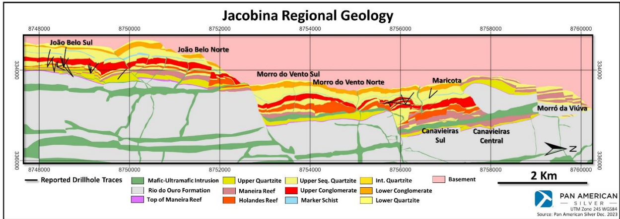
Figure 1. Jacobina - Regional Geology
