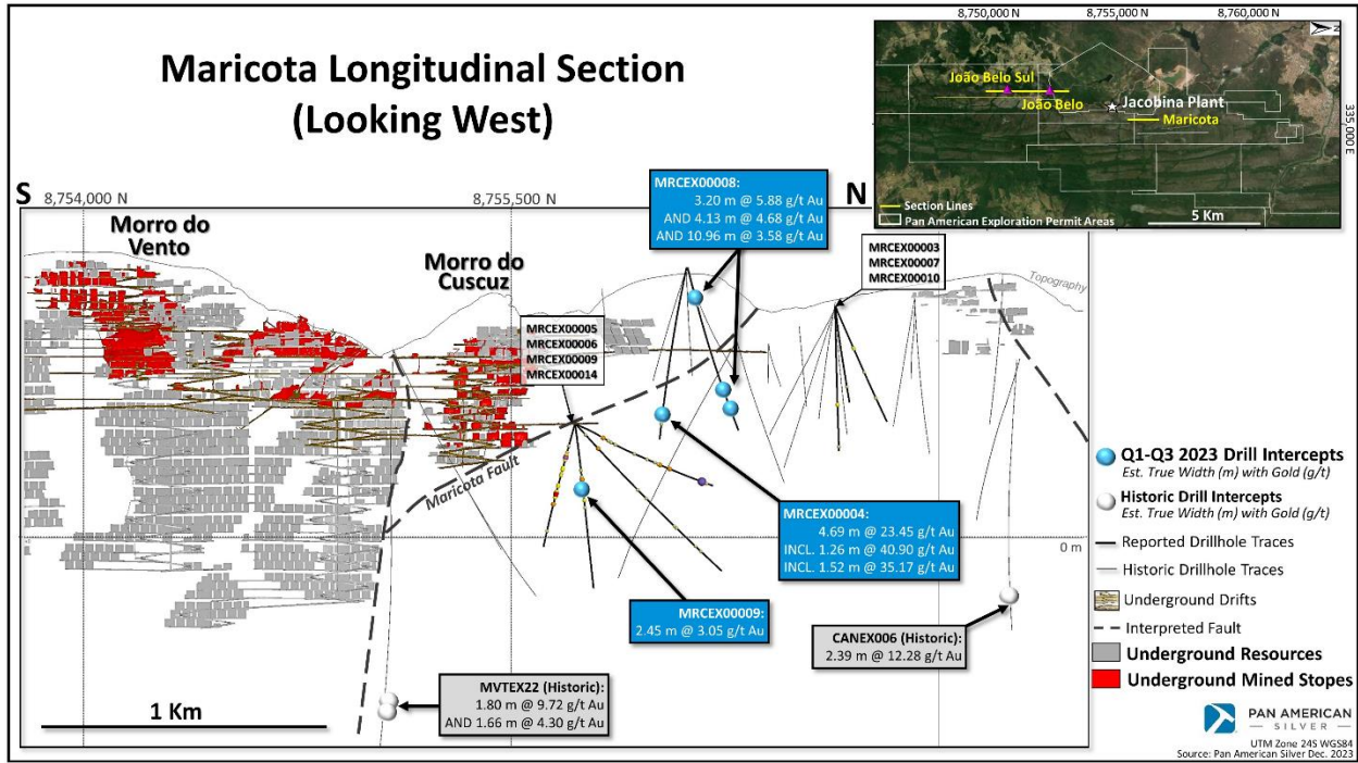
Figure 3. Jacobina - Maricota Main Reef Long Section
